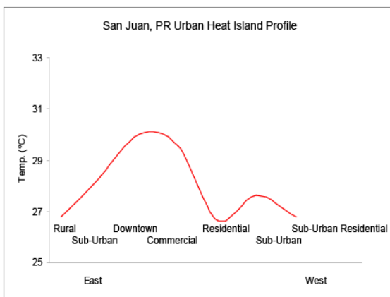
Figure 1 Schematic of the profile of temperatures typically observed in the San Juan Metropolitan Area.
