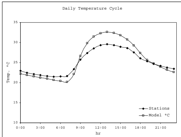
Figure 4 Comparison of the air temperatures between the regional model results and the stations and sensors deployed in the San Juan Metropolitan area.
